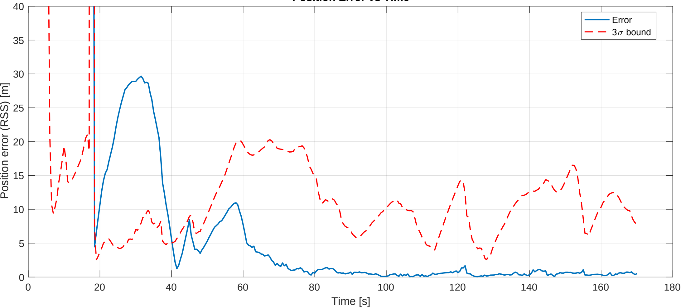
Position Error vs Time
